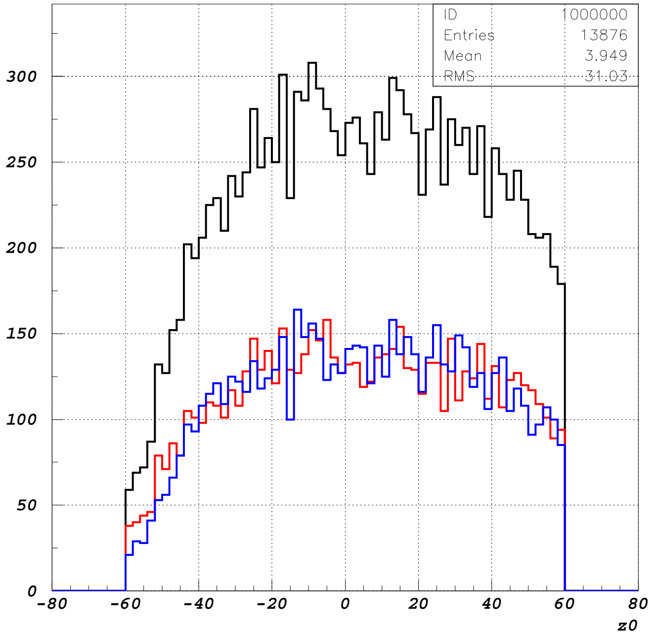
tazthickz15gev
