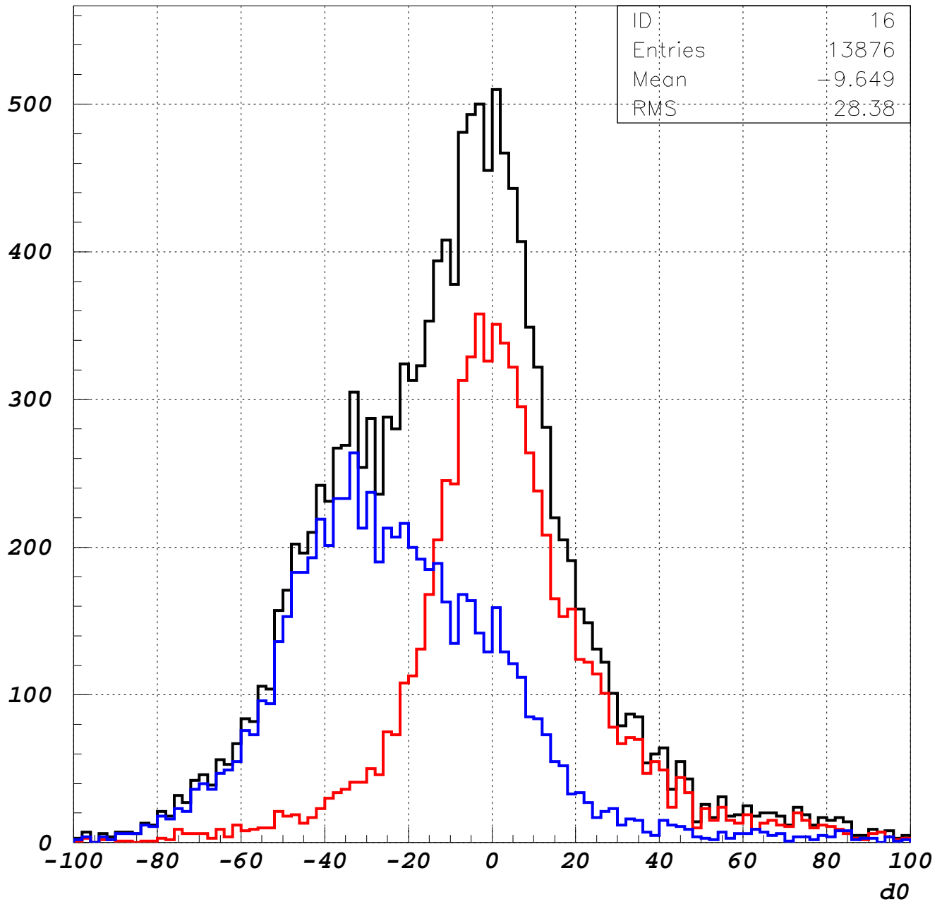
tazthickz15gev
